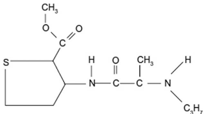
Fig.1. The chemical structure of articaine.
