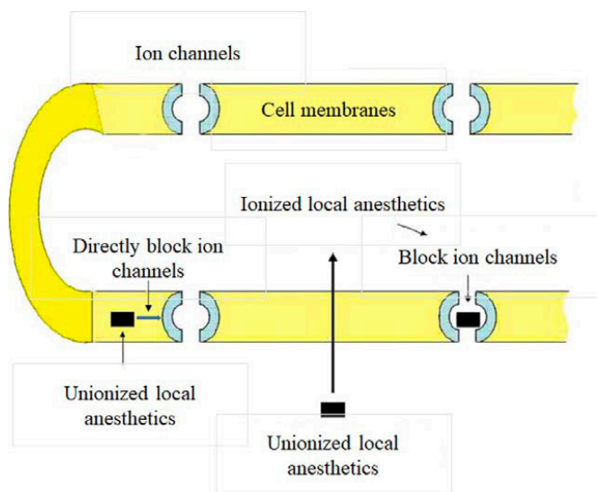
Fig.2. The mechanism of action of local anesthetics including articaine.
